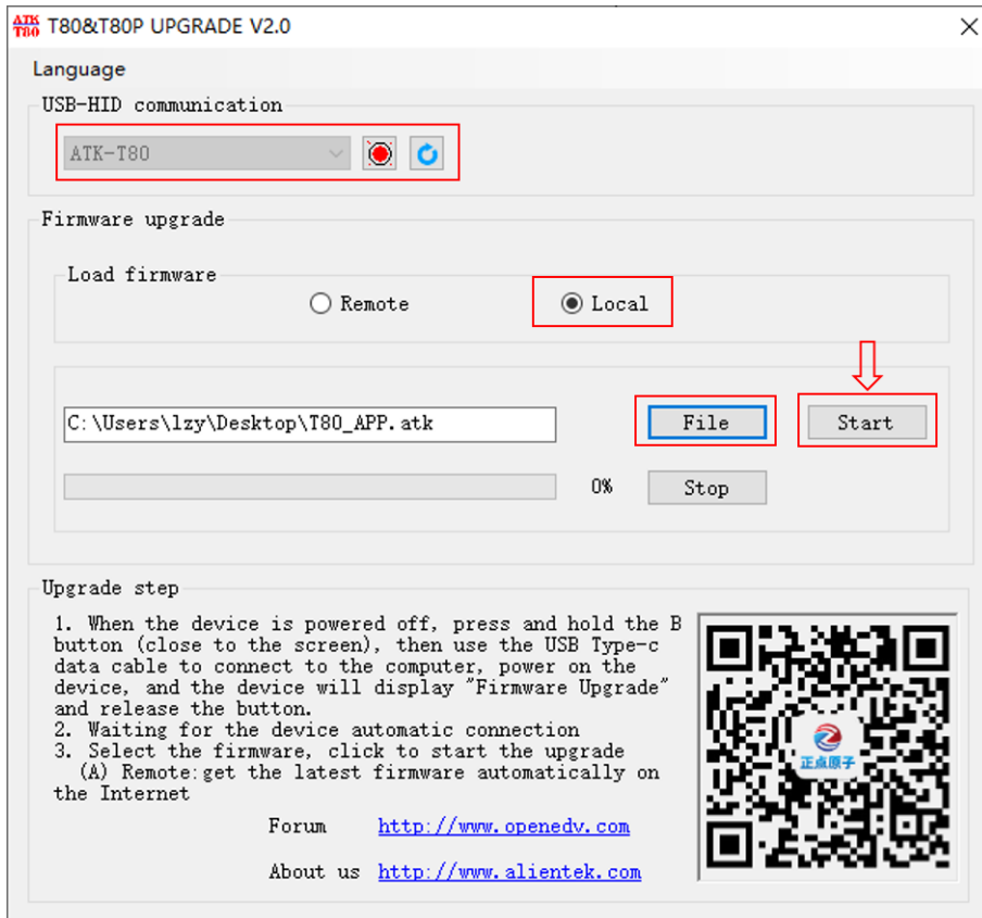
Figure 10-3 Firmware upgrade
