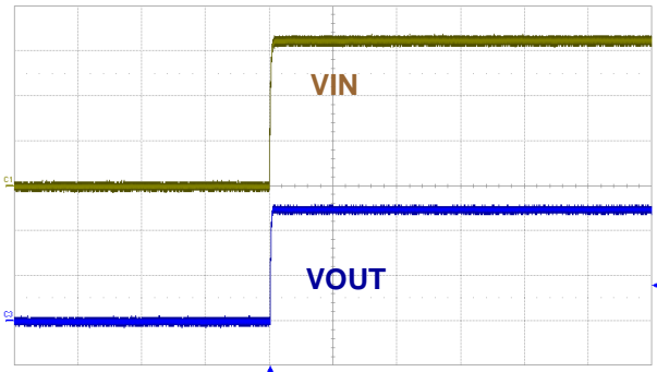
VIN: 1.0V/div, VOUT: 1.0V/div, Time: 10ms/div VIN=3.3V, VOUT=2.5V Start Up @ I_{OUT}=0.6A
