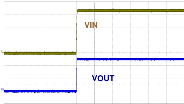
VIN: 1.0V/div, VOUT: 1.0V/div, Time: 10ms/div VIN=3.3V, VOUT=2.5V Start Up @ I_{OUT}=0.3A
