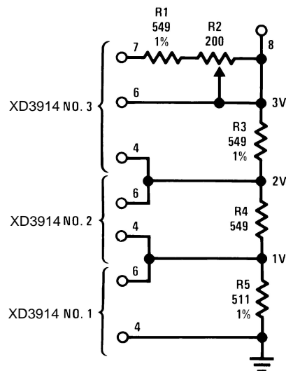
Figure 27. Adjusting Linearity of Several Stacked Dividers
