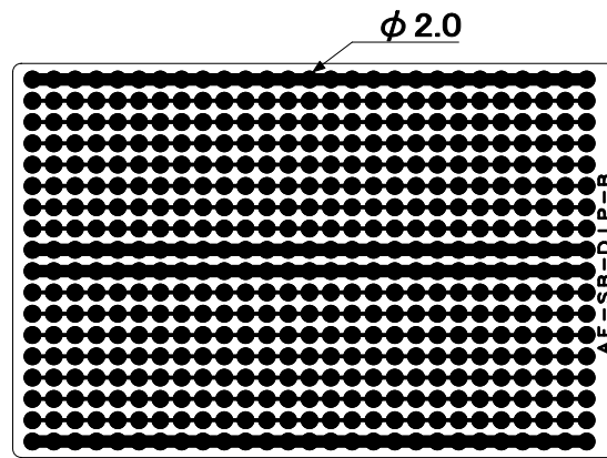
AE-SB-DIP-B L1-PATTERN
