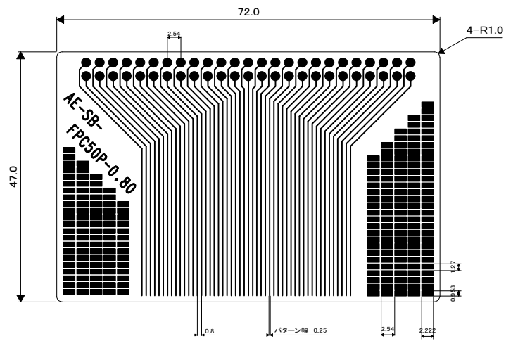
AE-SB-FPC50P-0.80 L1-PATTERN
