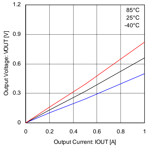
Fig.28 Output low voltage (BD6221/26)
