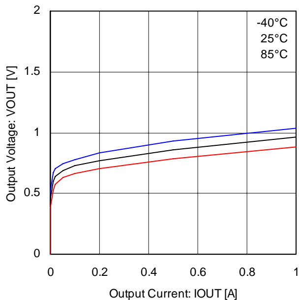
Fig.31 下側 Di 特性(BD6221/26)
