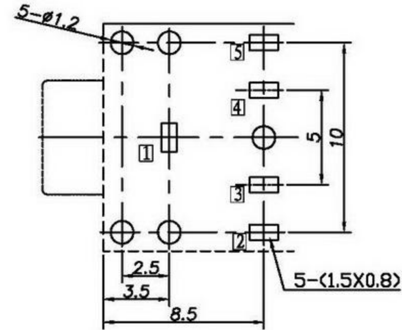
P. C. B Layout (Printed-sided view)
