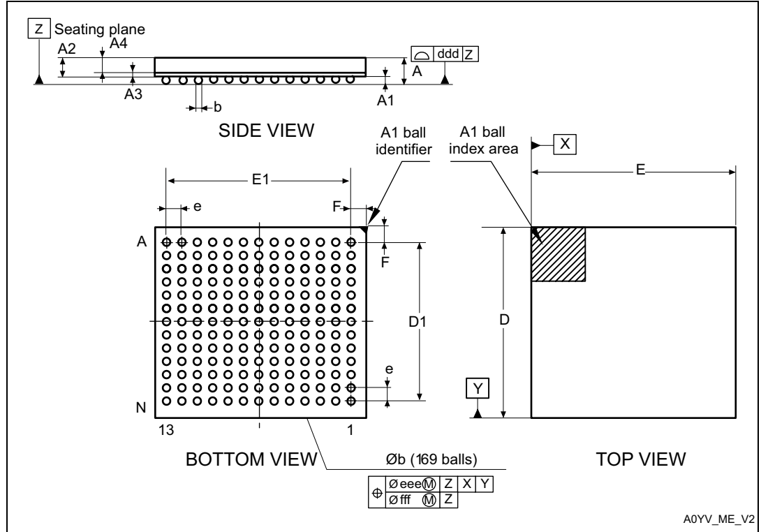
Figure 103. UFBGA169 - Outline
