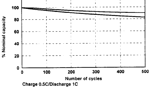
Cycle life curve of NiMH cylindrical cell
